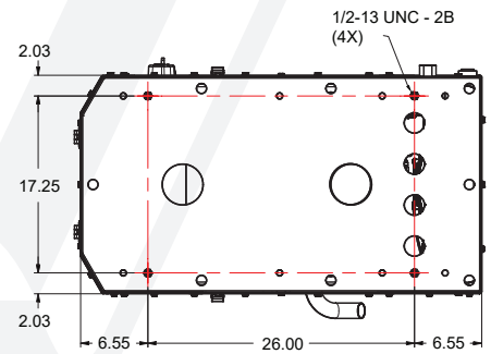
MOUNTING HOLES
